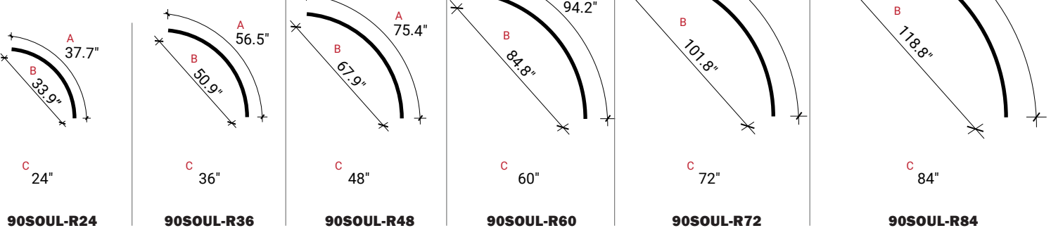
90 Degrees A. Curve length / B. Chord Length / C. Radius
