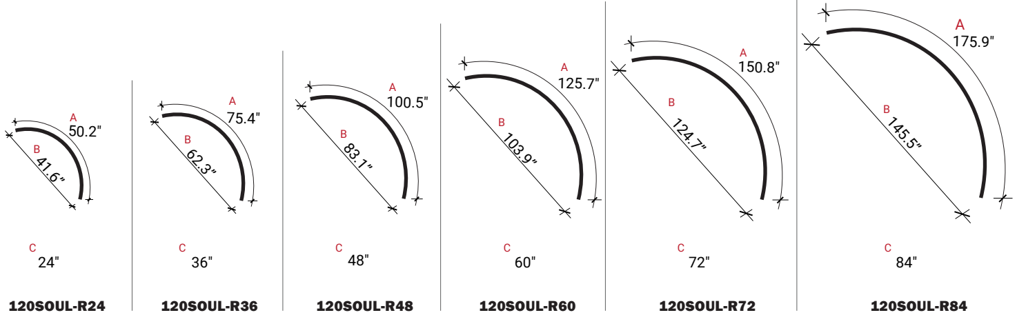
120 Degrees A. Curve length / B. Chord Length / C. Radius
