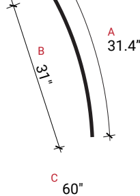
30SOUL-R60
