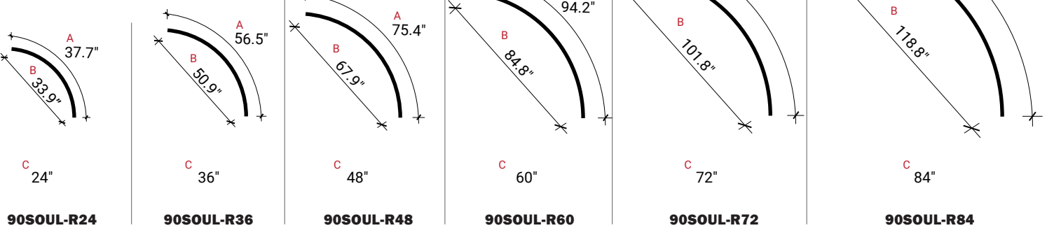
90 Degrees A. Curve length / B. Chord Length / C. Radius
