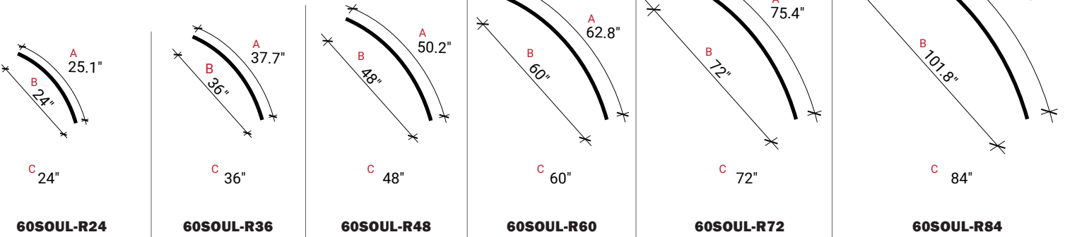
60 Degrees A. Curve length / B. Chord Length / C. Radius
