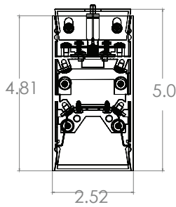
2" PROFILE
