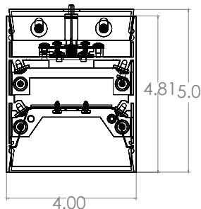
4" PROFILE
