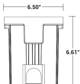
MOUNTING SLEEVE
