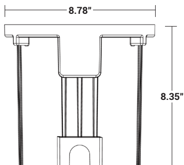
MOUNTING SLEEVE
