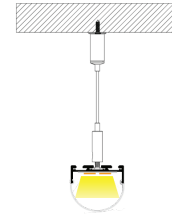
Profiles with suspended cable mounting
