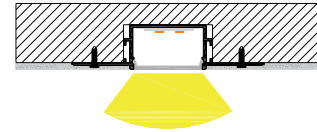
Trimless mounting
