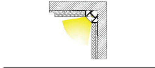
Mounting the profile directly behind the tile.
