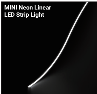
Series-LB1004-ST 380lm/ft - 6W/ft Indoor Strip Light Width / 0.39" / 10mm 128 LEDs/FT
