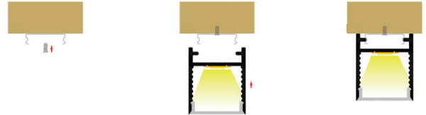
Profile with surface mounting clip
