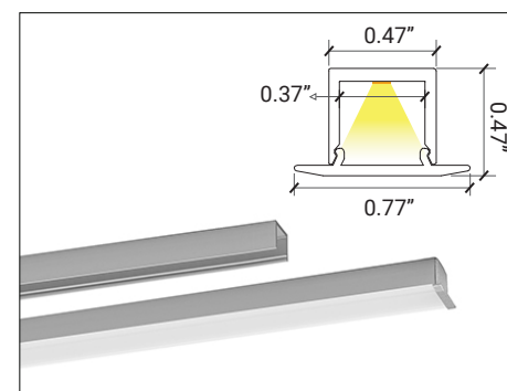
LP-LGC-RFT-050/ Recessed
