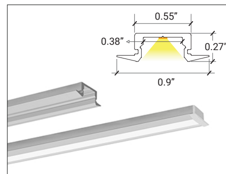
LP-MDC-RFT-050/ Recessed
