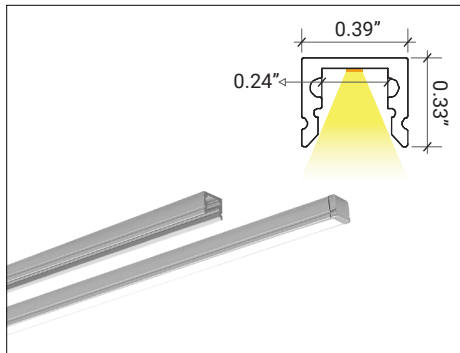
LP-MDC-CM-025/ Surface
