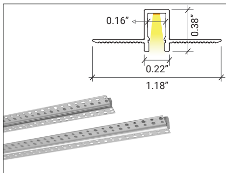
LP-MDC-RTL-025/ Trimless
