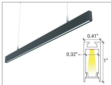
LP-LGC-SPD-1/ Suspended
