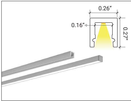
LP-SHC-CM-025/ Surface
