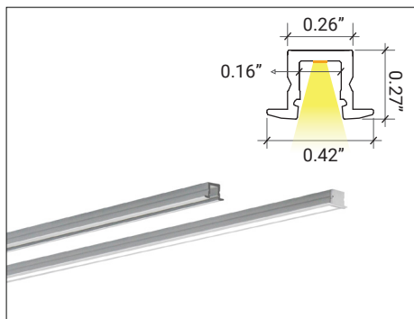
LP-MDC-RFT-025/ Recessed
