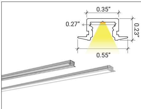
LP-SHC-RFT-025/ Recessed
