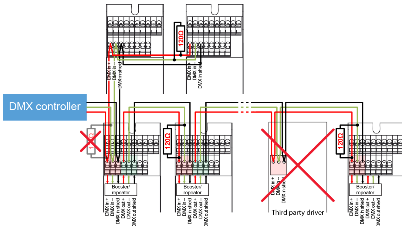
Figure 7 – It is not possible to have third party drivers in the DMX out-chain
