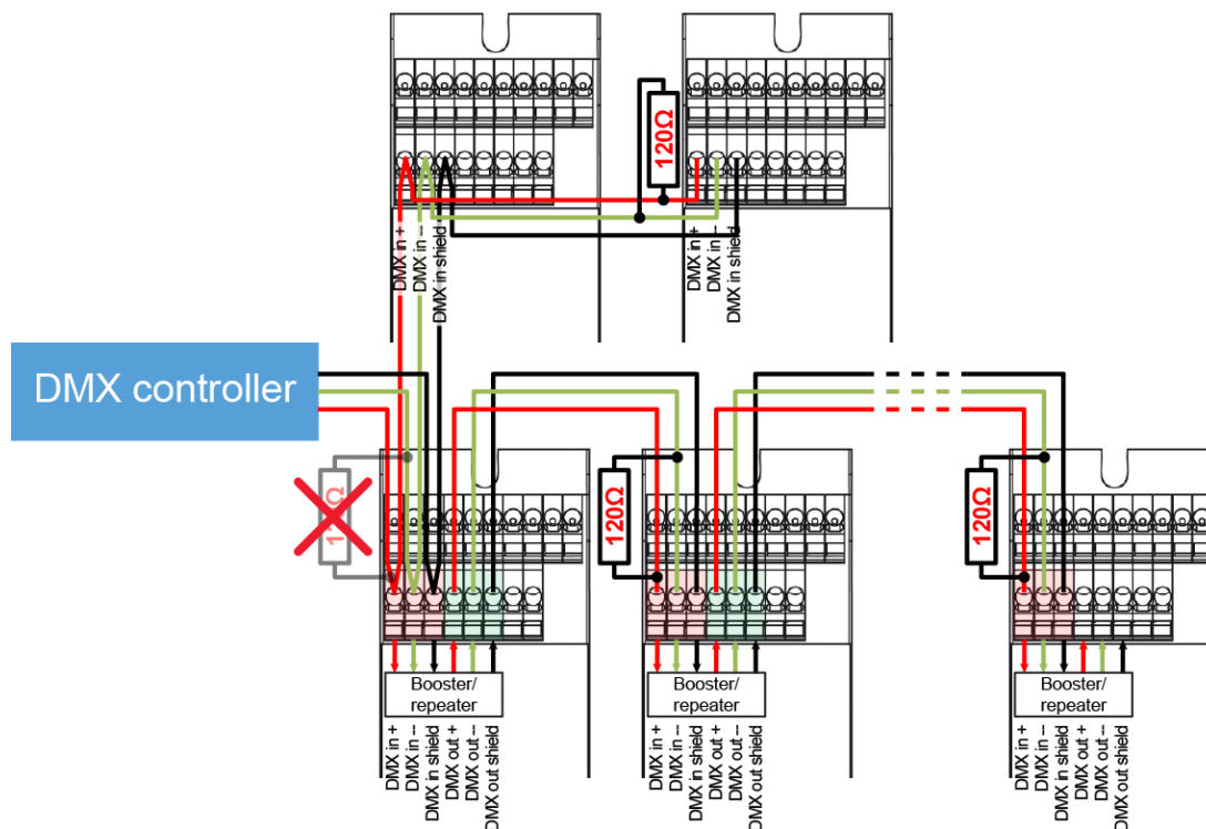
Figure 6 Mixed topology with daisy chain and DMX out
