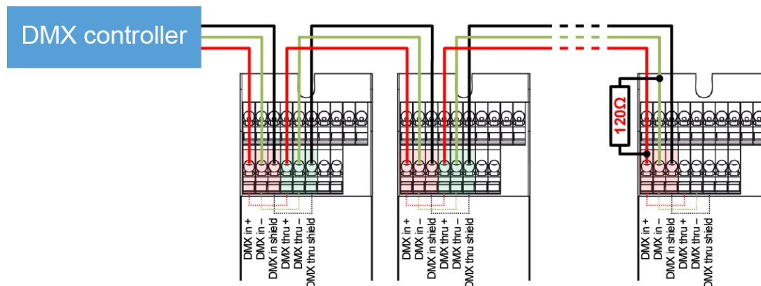
Figure 4 – Daisy chain topology with 'DMX in' and 'DMX thru'
