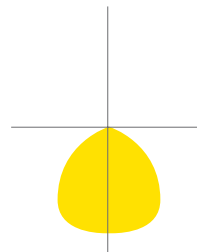
Wide Flood (WFL) Candle Power Distribution Curve
