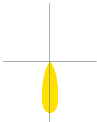
Spot (SP) Candle Power Distribution Curve
