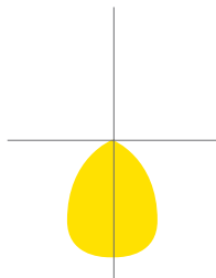
Flood (FL) Candle Power Distribution Curve
