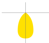
Narrow Flood (NFL) Candle Power Distribution Curve
