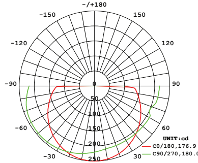
AVERAGE BEAM ANGLE (50%): 178.4 DEG
