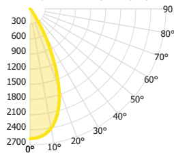
CANDELA DISTRIBUTION
