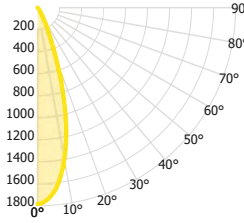
CANDELA DISTRIBUTION
