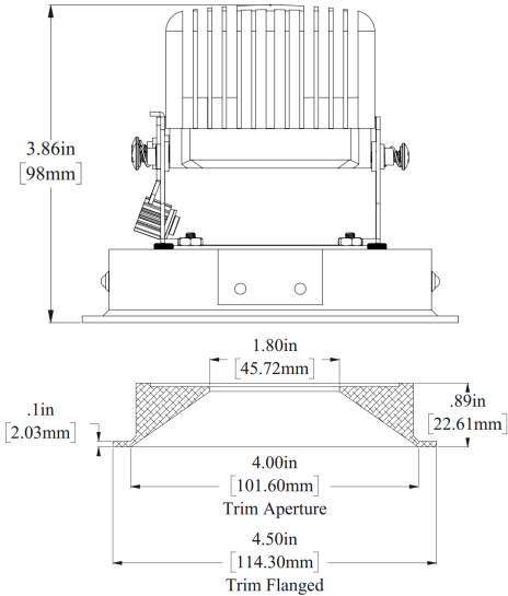
FCD-SQ4-F-1302/1328 Flanged
