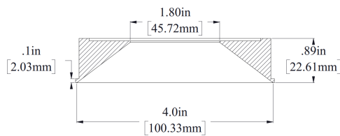
FCD-SQ4-TL-1302/1328 Trimless/Millwork
