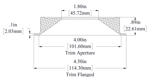
FCD-SQ4-F-1302/1328 Flanged
