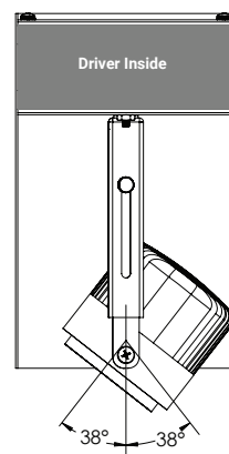
Head 38-degree rotation capability. (Head inside the housing)
