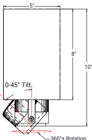
Head 45-degree rotation capability. (Head outside the housing)
