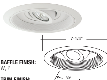
B1619W-WH ADJUSTABLE SPOT (30° TILT)
