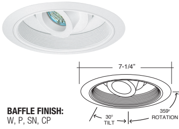
B1601W-WH ADJUSTABLE SPOT (30° TILT)
