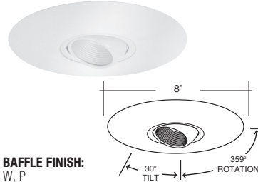
B1661W-WH ADJUSTABLE EYEBALL
