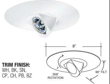
B1605WH SURFACE ADJUSTABLE (90° TILT)
