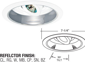
B1656CL-WH REFLECTOR (30° TILT)
