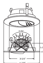
B1418P-WH ADJ.PINHOLE W/ EYEBALL (35° TILT)
