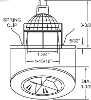
B1262RG-WH REFLECTOR SHOWER TRIM
