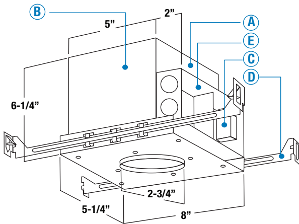
CEILING ACCESS REQUIRED TO SERVICED TRANSFORMER
