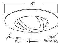
B684RG-WH PAR38 REFLECTOR W/ GIMBAL RING
