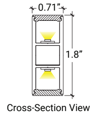
Cross-Section View
