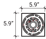
Mounting Plate
