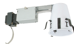
BL4R-50-M-120-AT 4" Miniature Low Voltage Non-IC Remodel Housing with Magnetic Transformer
