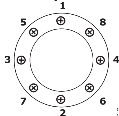
Order in which to tighten/remove screws
