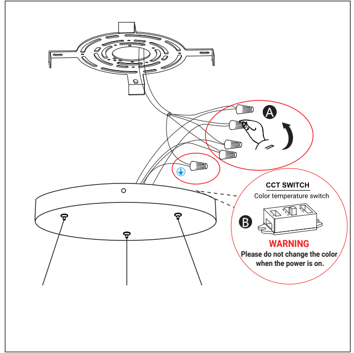
2 A. Connect the power wires and secure them with a connector cap. B. Choose the color temperature when the fixture is powered off.
