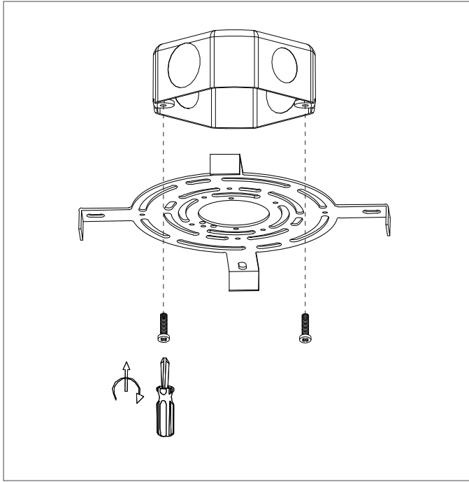
1 Secure the J-Box and mounting bracket with screws.
