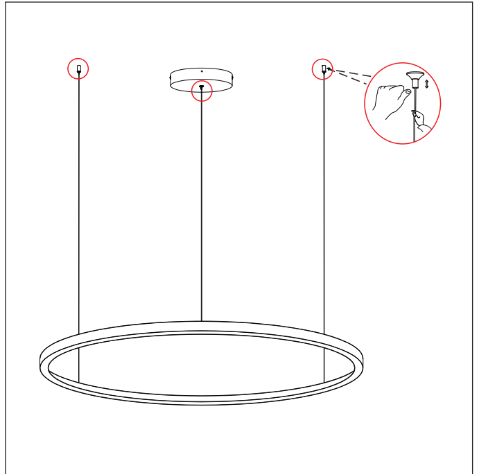
4 Press the suspension pin to adjust the fixture height.
