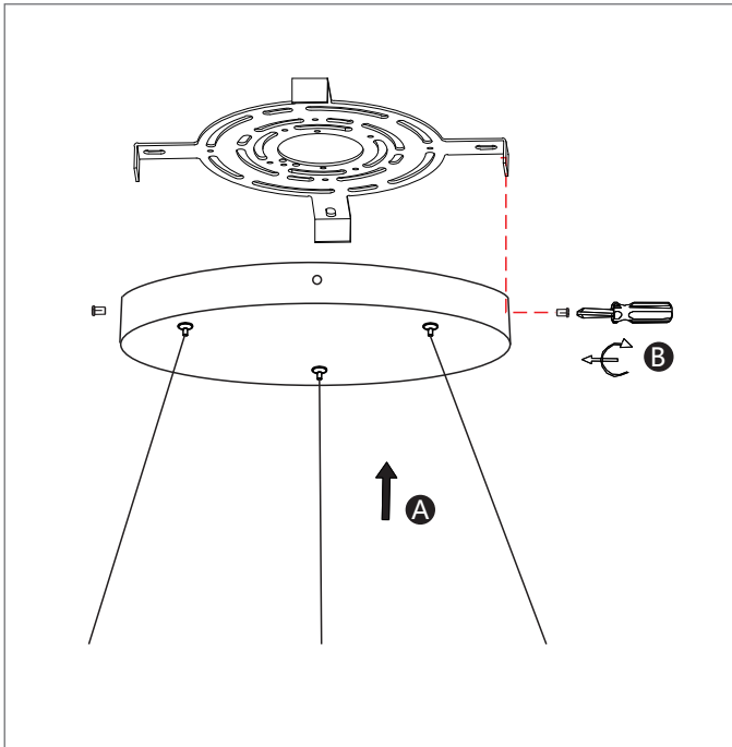
3 Attach and secure the canopy to the bracket with screws.
