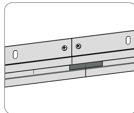
Step 5: Screw in the next fixture into the bracket
